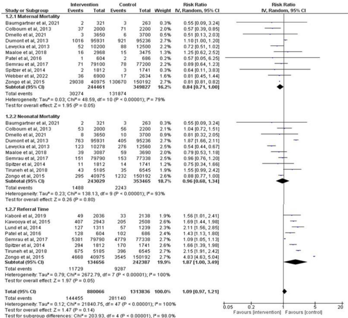
Forest Plot
